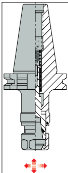
GTI DIN69871 Page 956
