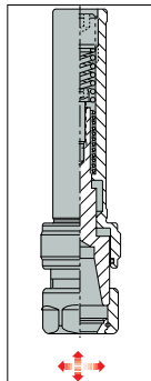
Straight Shank Page 1056
