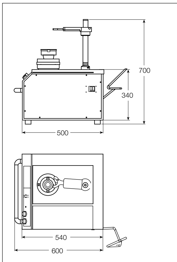
Trolley (optional)
