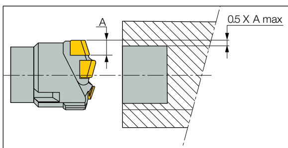
Recommended Coolant Pressure and Volume \leq 50 mm
