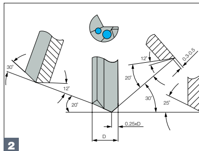
2 Standard sharpening for 4 to 32 mm drill diameters
