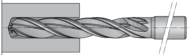
1 3 flute drill, drilling a pre-hole (drill diameter +0.02 mm)
