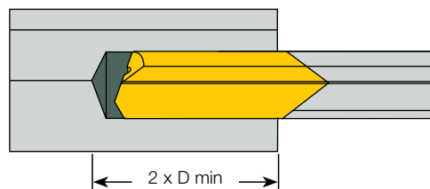
2 Gundrill penetration through the pre-hole
