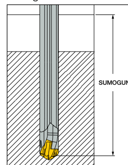
4. Continue drilling at recommended cutting conditions
