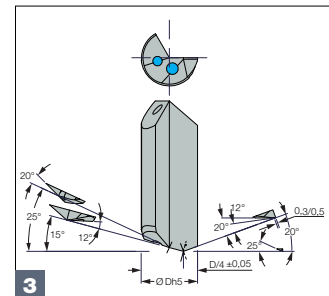
3 Standard sharpening for 32 to 40 mm drill diameters
