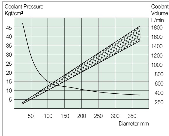
Recommended Coolant Pressure and Volume > 50 mm
