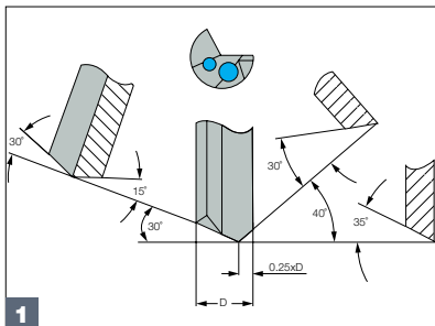
1 Standard sharpening for 0.9 to 4 mm drill diameters
