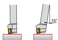
PFXN(RL) EXT
