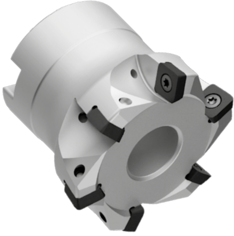
Weldon Shank K r =10° | γ p =+2° | γ f =+2° | R p =0.079
