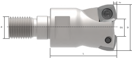
SCREW COUPLING - SDKX 0904-HF / SDKW 0904-HF
